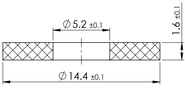
SECTION X-X
